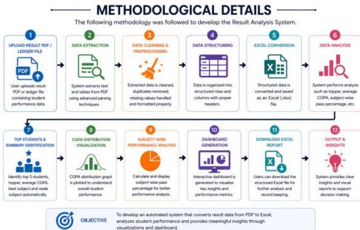
Fig. 3: Methodology
